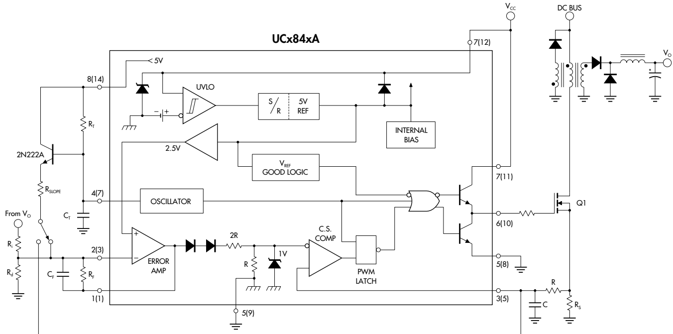
FIGURE 6. — SLOPE COMPENSATION
