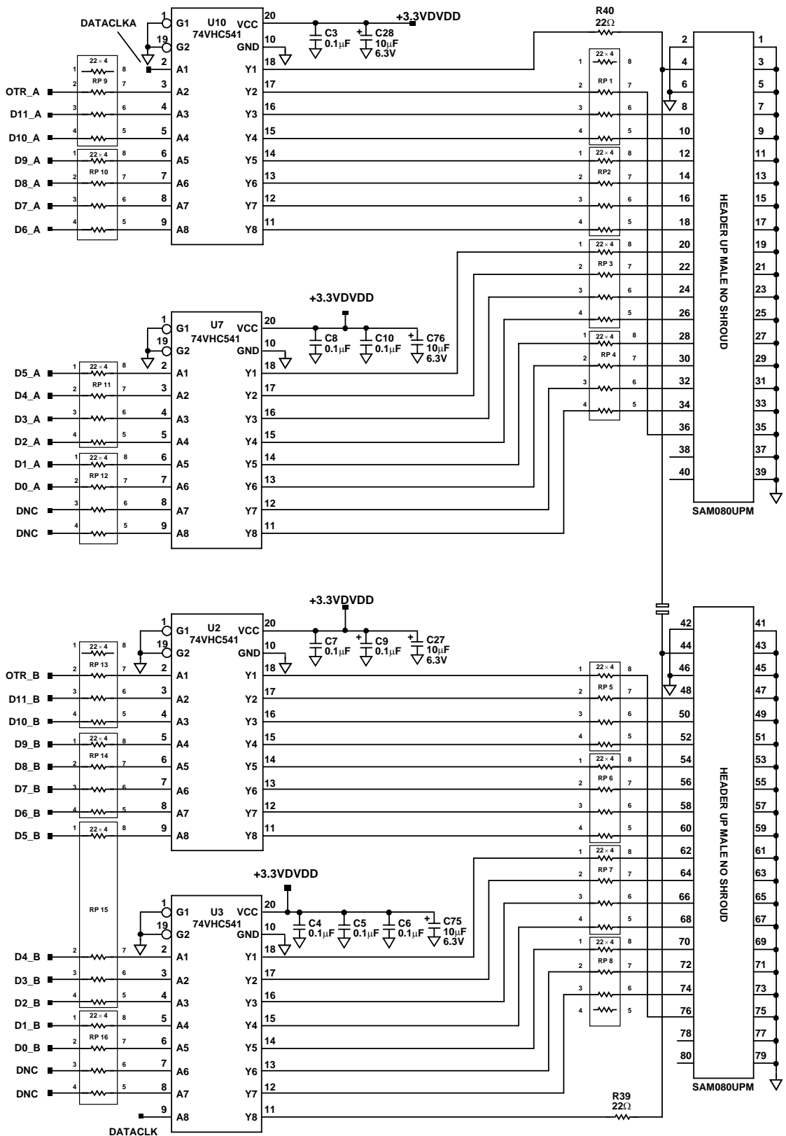
Figure 78. Interface Schematic
