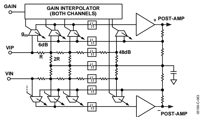
Figure 63. Simplified VGA Schematic
