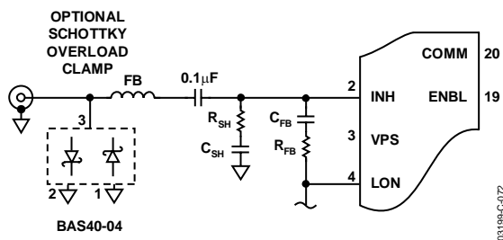
Figure 73. Input Overload Clamping
