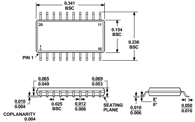
COMPLIANT TO JEDEC STANDARDS MO-137AD
