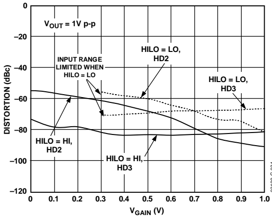
Figure 34. Harmonic Distortion vs. V_GAIN, f = 10 MHz
