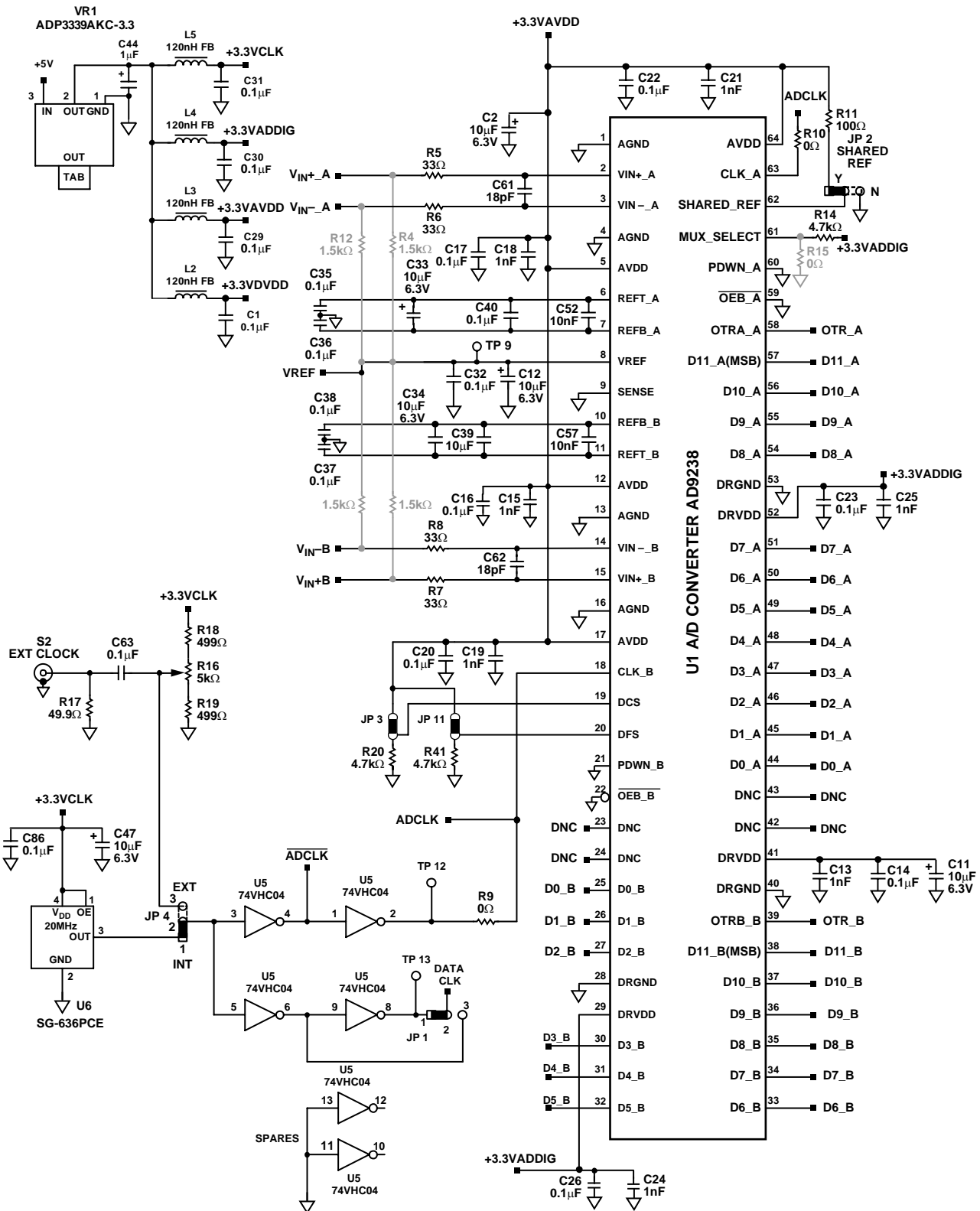
Figure 77. Converter Schematic
