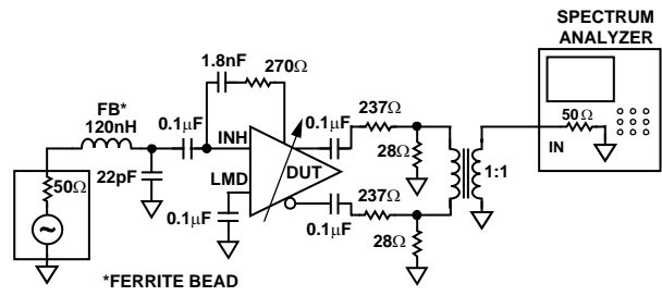
Figure 54. Distortion
