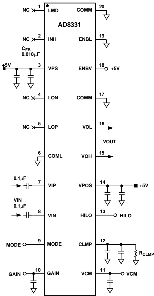
Figure 74. Disabling the LNA
