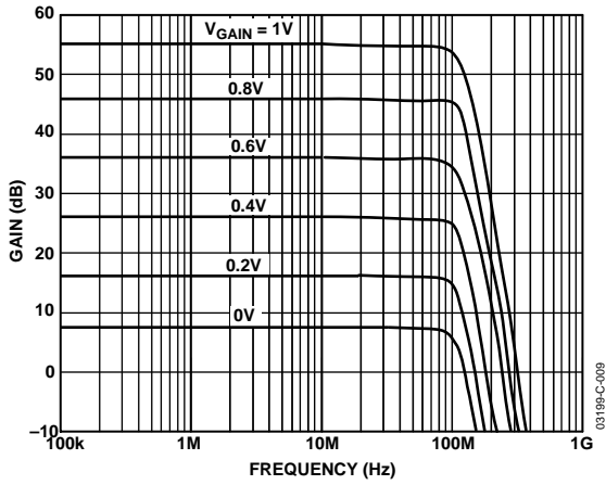
Figure 9. Frequency Response for Various Values of V_{GAIN} , HILO = HI
