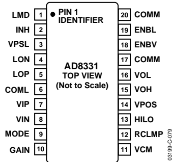
Figure 79. 20-Lead QSOP
