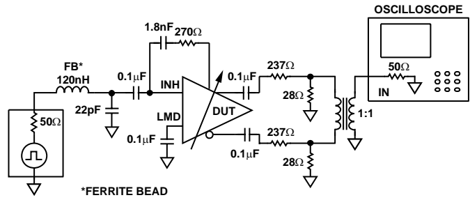
Figure 52. Transient Measurements
