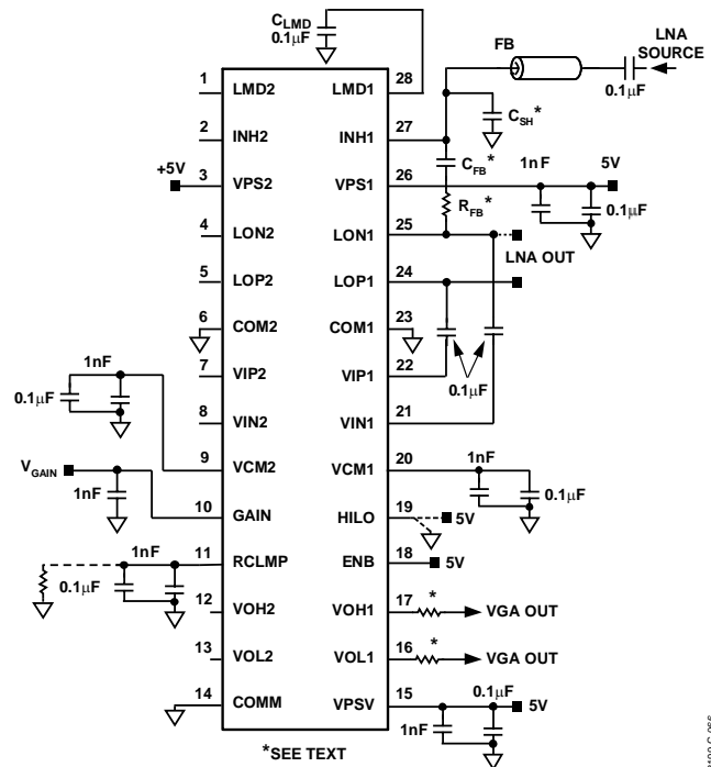
Figure 66. Basic Connections for a Typical Channel (AD8332 Shown)
