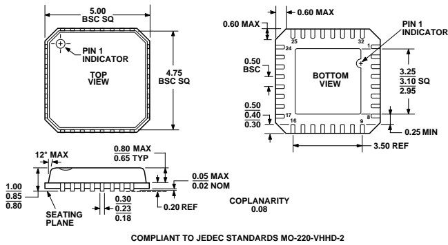
COMPLIANT TO JEDEC STANDARDS MO-220-VHHD-2
