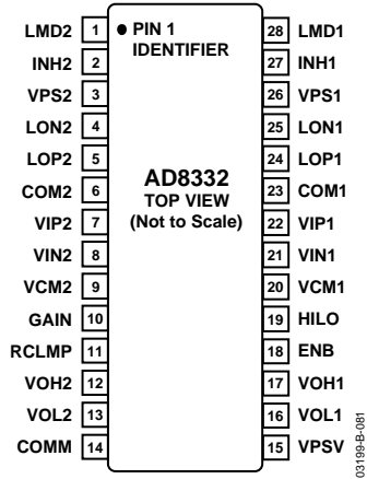
Figure 80. 28-Lead TSSOP
