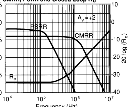
CMRR, PSRR and Closed Loop R_o
