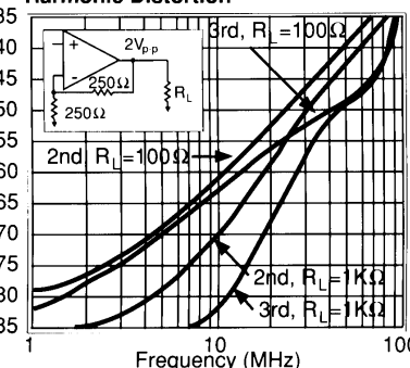
2nd Harmonic Distortion
