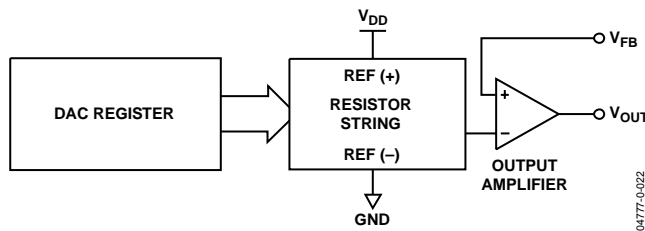
Figure 27. DAC Architecture
