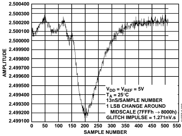
Figure 22. Digital-to-Analog Glitch Impulse (Positive)
