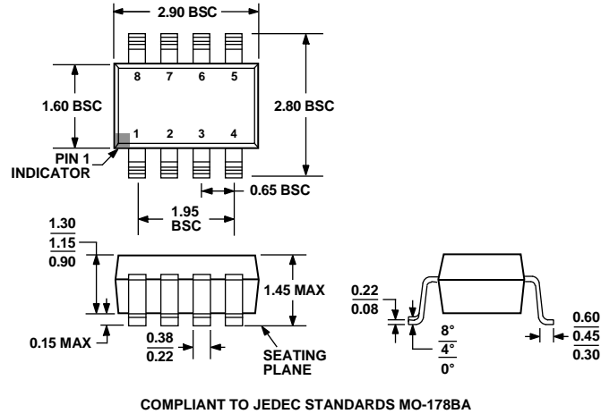
Figure 39. 8-Lead SOT-23 (RJ-8) Dimensions shown in millimeters
