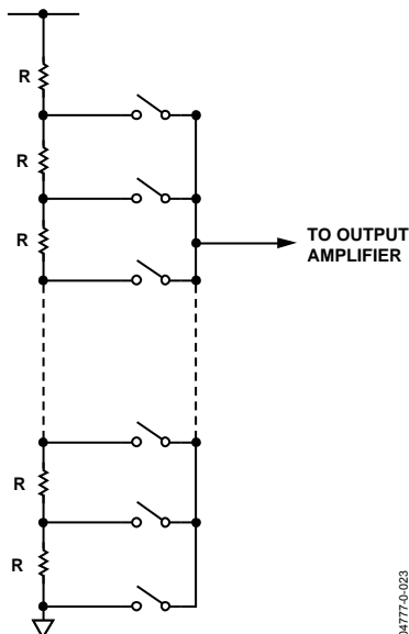
Figure 28. Resistor String
