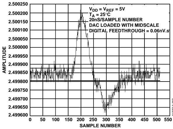
Figure 23. Digital Feedthrough
