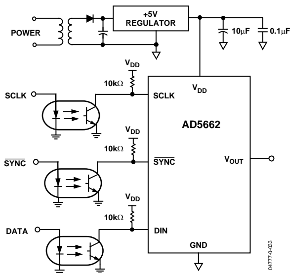
Figure 38. AD5662 with an Opto-Isolated Interface
