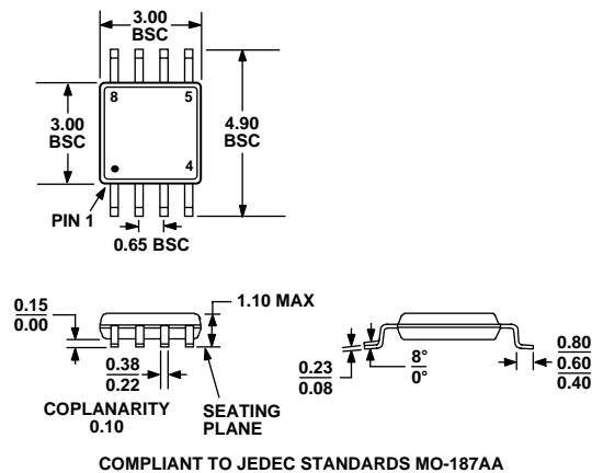
Figure 40. 8-Lead Mini Small Outline Package [MSOP] (RM-8) Dimensions shown in millimeters
