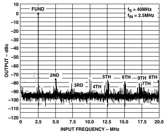
Figure 10. FFT Response for AD8132 Driving AD9203
