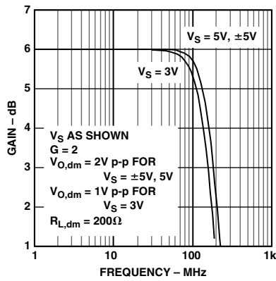
TPC 13. Large Signal Frequency Response
