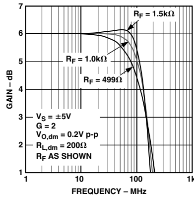
TPC 14. Small Signal Frequency Response vs. R_F
