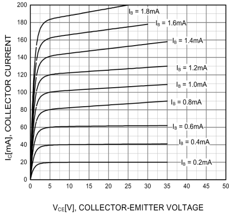
Figure 1. Static Characteristic
