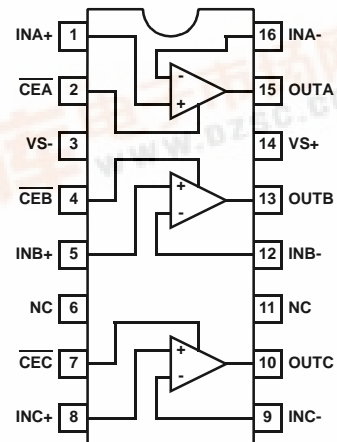
EL5393A [16-PIN SO (0.150"), QSOP] TOP VIEW
