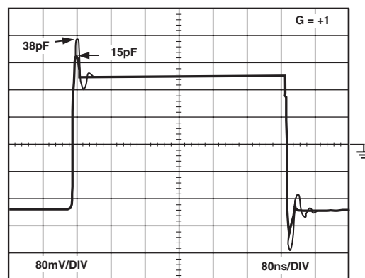
TPC 22. Small Signal Transient Response \pm 5 V (See Test Circuit 1)
