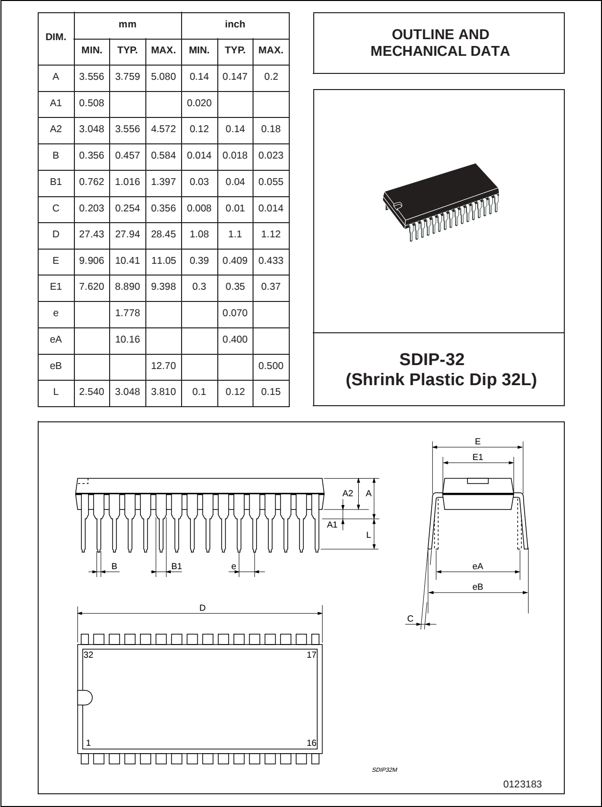
Figure 18. SDIP-32 Mechanical Data & Package Dimensions
