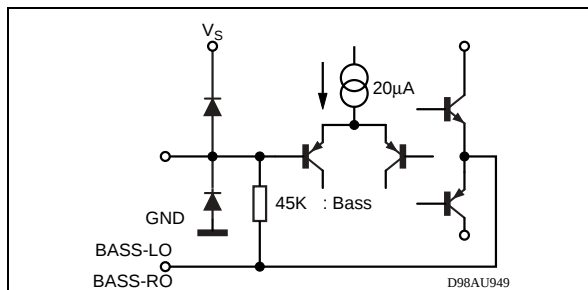
Figure 15. PIN: BASS-LI, BASS-RI
