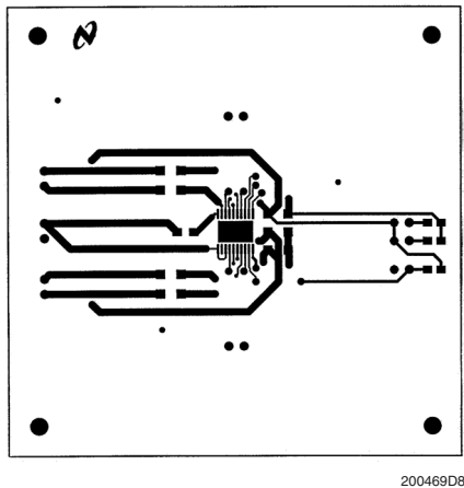
FIGURE 3. Recommended MH PC Board Layout: Component-Side Layout
