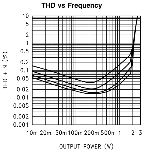
V_{DD} = 5V , R_L = 3\Omega , f_{IN} = 1kHz , at (from top to bottom at 50mW): A_V = 21.6dB , A_V = 15.6dB , A_V = 10dB , A_V = 6dB
