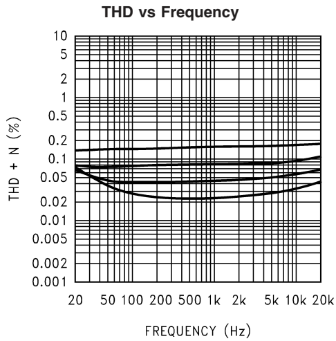
V_{DD} = 5V , R_L = 8\Omega , P_{OUT} = 400mW , at (from top to bottom at 1kHz): A_V = 21.6dB , A_V = 15.6dB , A_V = 10dB , A_V = 6dB
