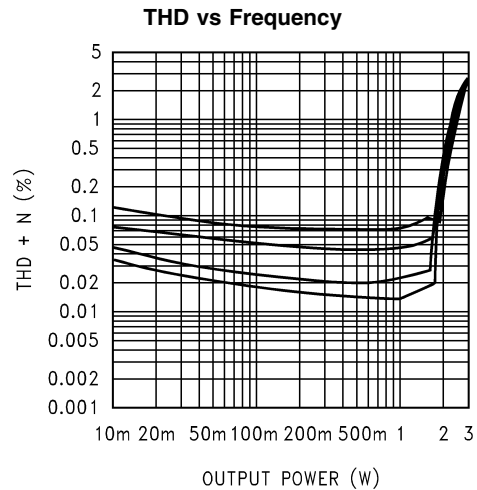
V_{DD} = 5V , R_L = 3\Omega , f_{IN} = 20kHz , at (from top to bottom at 50mW): A_V = 21.6dB , A_V = 15.6dB , A_V = 10dB , A_V = 6dB
