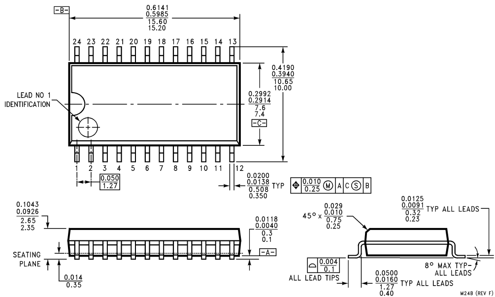
Order Number DS14C238WM NS Package Number M24B
