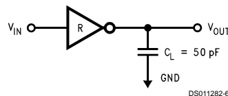
FIGURE 3. Receiver Load Circuit
