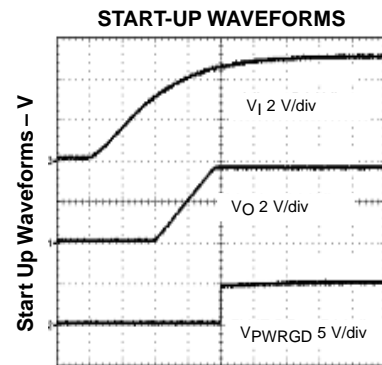
Time – 2 ms/div
