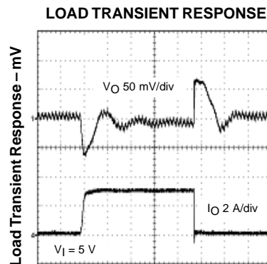
Time – 10 μs/div
