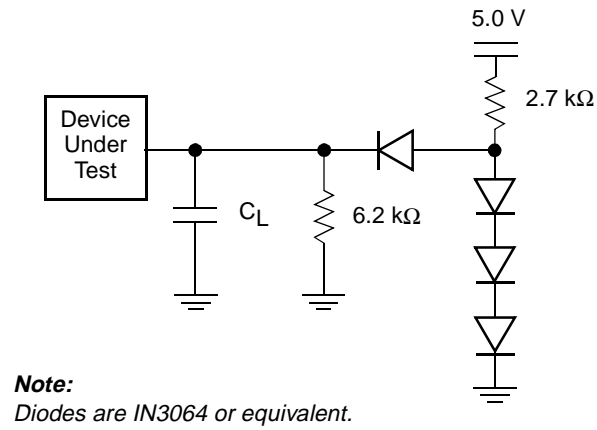
Figure 8. Test Setup
