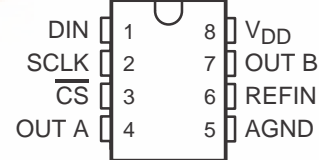
D PACKAGE (TOP VIEW)
