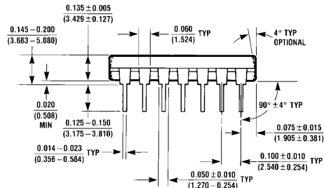
Molded Dual-In-Line Package (N) Order Number LM361N NS Package Number N14A
