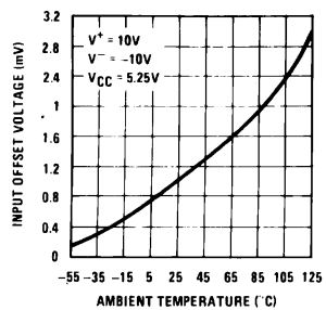
Offset Voltage
