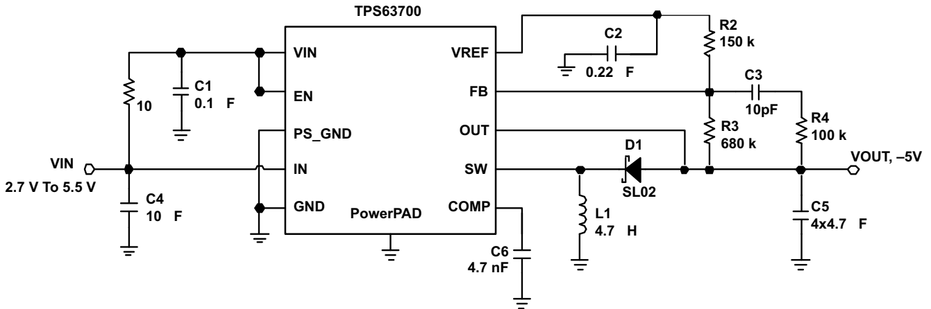
Figure 14. Circuit for –5 Volt Output
