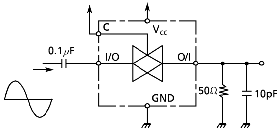
6. FREQUENCY RESPONSE (SWITCH ON)
