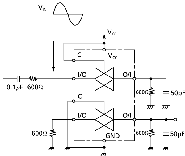
5. CROSSTALK (BETWEEN ANY TWO SWITCHES)
