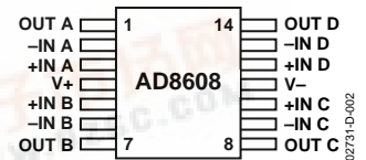
Figure 6. 14-Lead TSSOP (RU Suffix)
