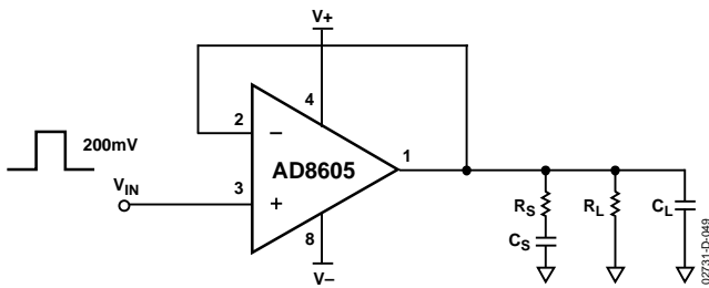
Figure 48. Snubber Network Configuration
