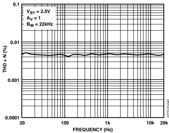
Figure 45. THD + N
