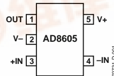
Figure 1. 5-Lead SOT-23 (RT Suffix)
