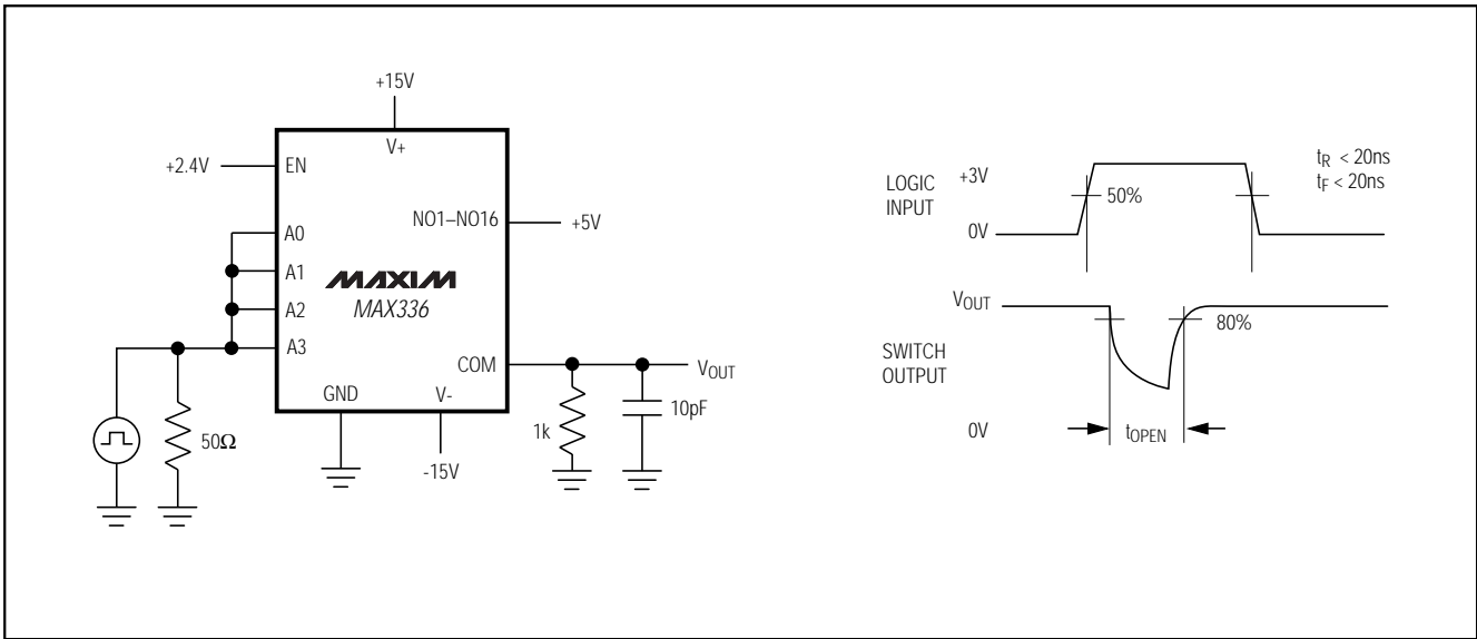
Figure 4. Break-Before-Make Interval
