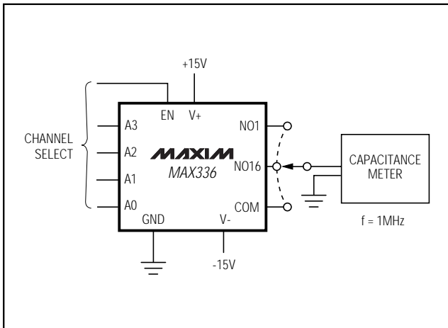
Figure 8. NO/COM Capacitance
