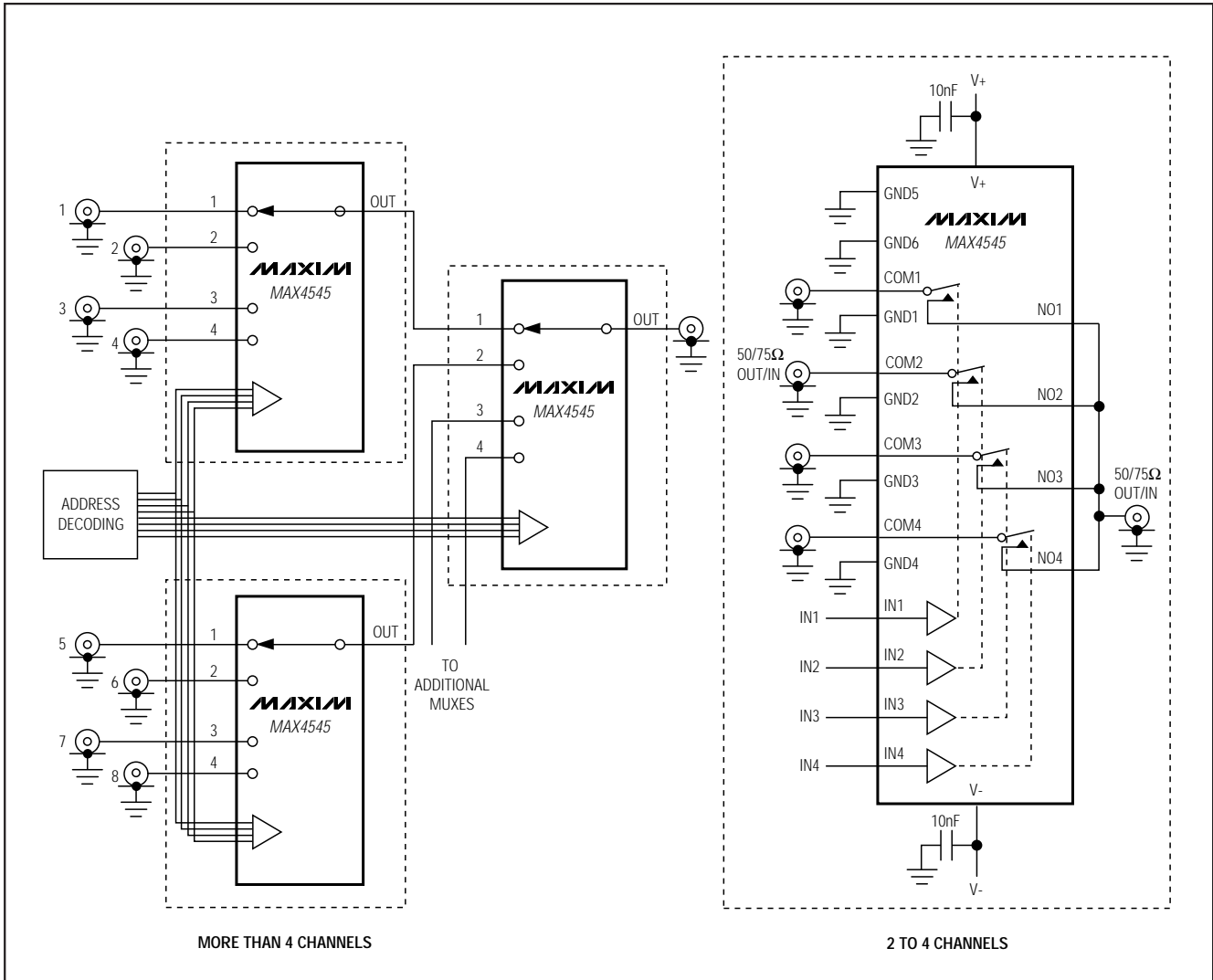
Figure 3. 4-Channel Multiplexer
