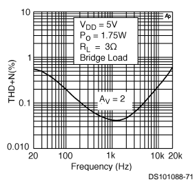
LM4836MTE THD+N vs Frequency
