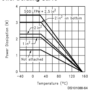
LM4836MTE (Note 17) Power Derating Curve
