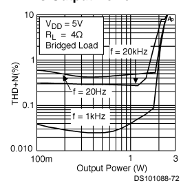
LM4836MTE THD+N vs Output Power
