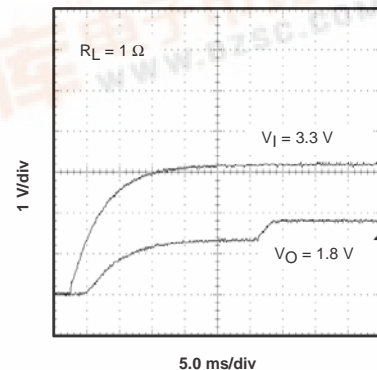
START UP WAVEFORM
