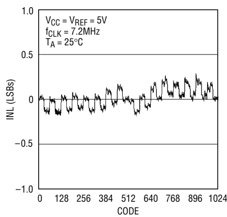
INL Plot
