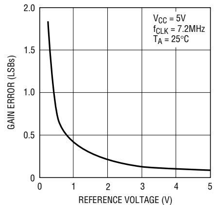
LTC1197 Gain Error vs Reference Voltage
