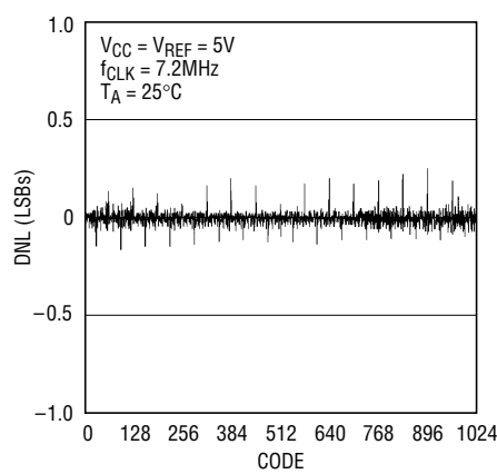
DNL Plot
