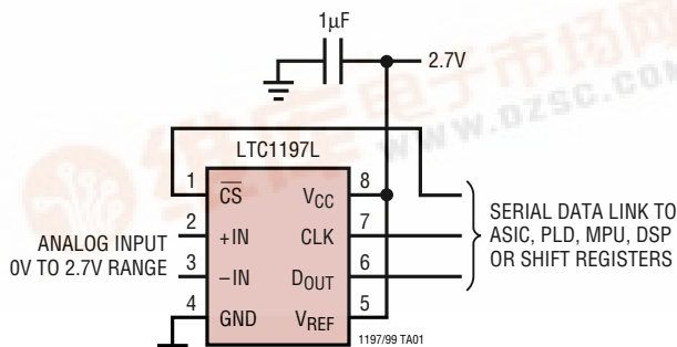
Single 2.7V Supply, 250ksps, 10-Bit Sampling ADC
