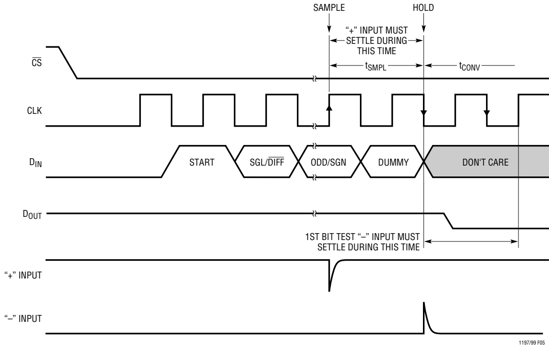
Figure 5. LTC1199/LTC1199L “+” and “-” Input Settling Windows
