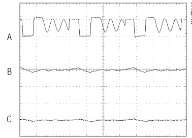
LIGHT-LOAD, PWM-MODE SWITCHING WAVEFORMS
