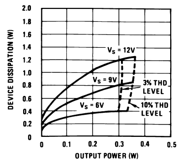
Device Dissipation vs Output Power—4 \Omega Load
