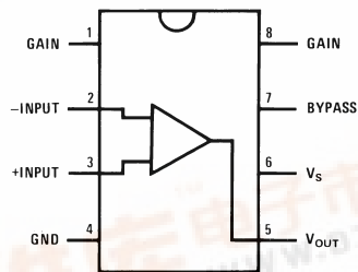
Small Outline,
