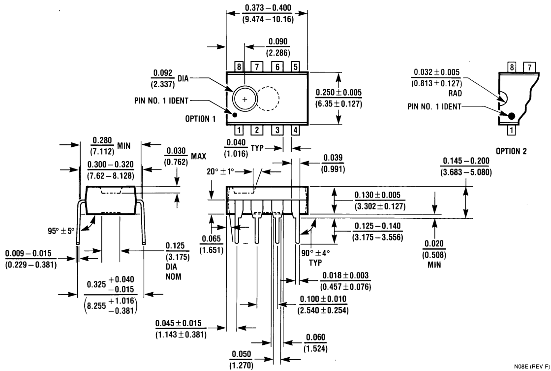
Dual-In-Line Package
