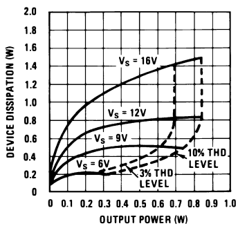
Device Dissipation vs Output Power—8 \Omega Load
