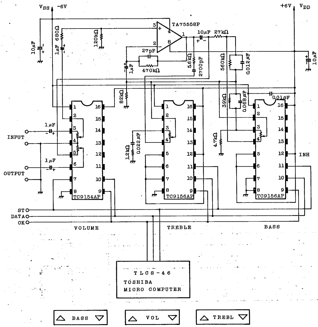
TC9154/56AP APPLICATION CIRCUIT (L-ch only)
