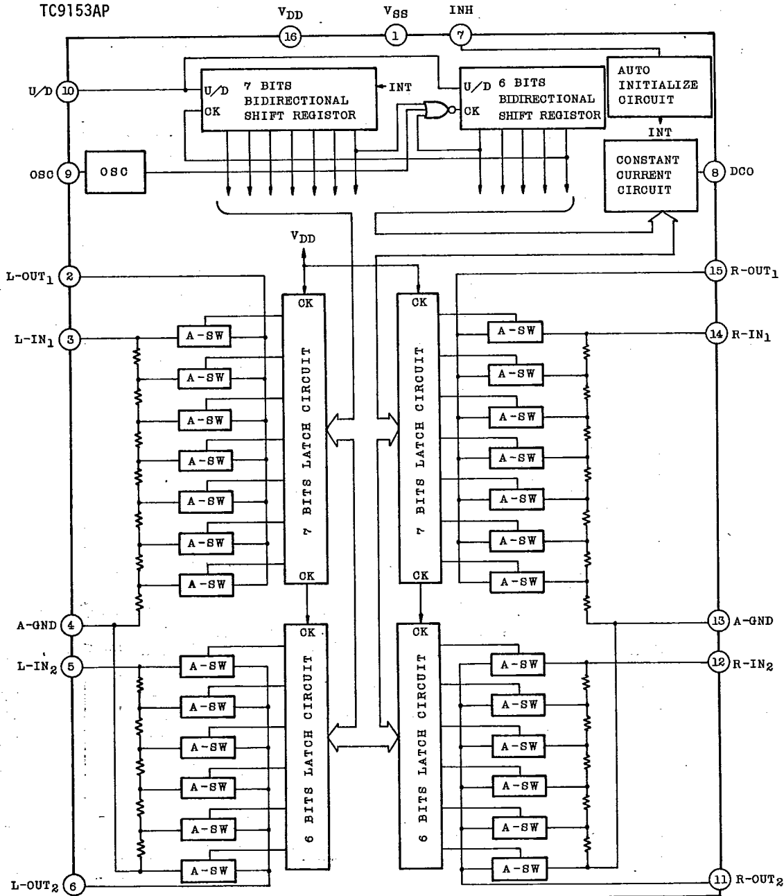
BLOCK DIAGRAM TC9153AP
