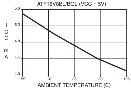
SUPPLY CURRENT vs. AMBIENT TEMPERATURE
