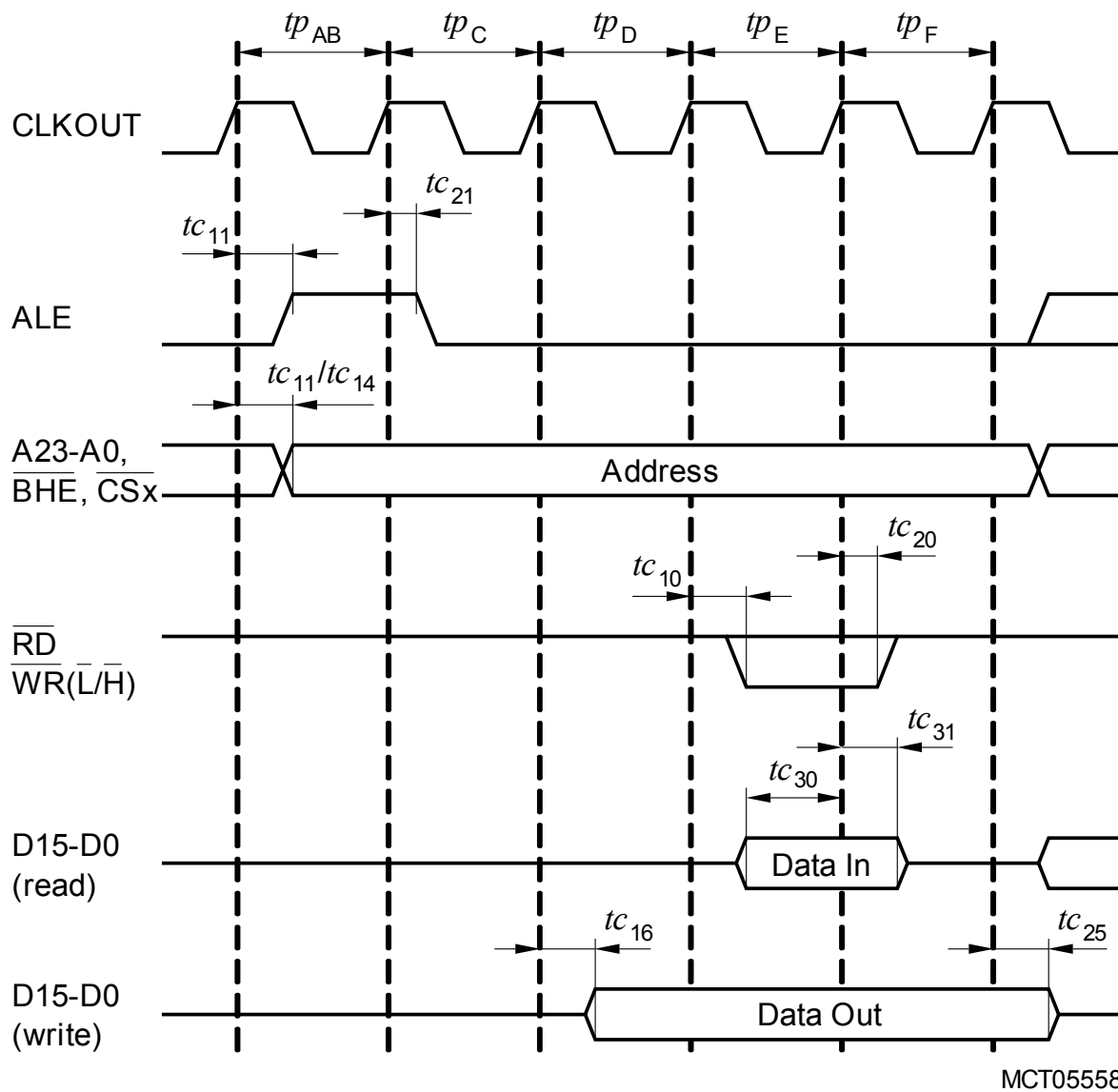
Figure 22 Demultiplexed Bus Cycle
