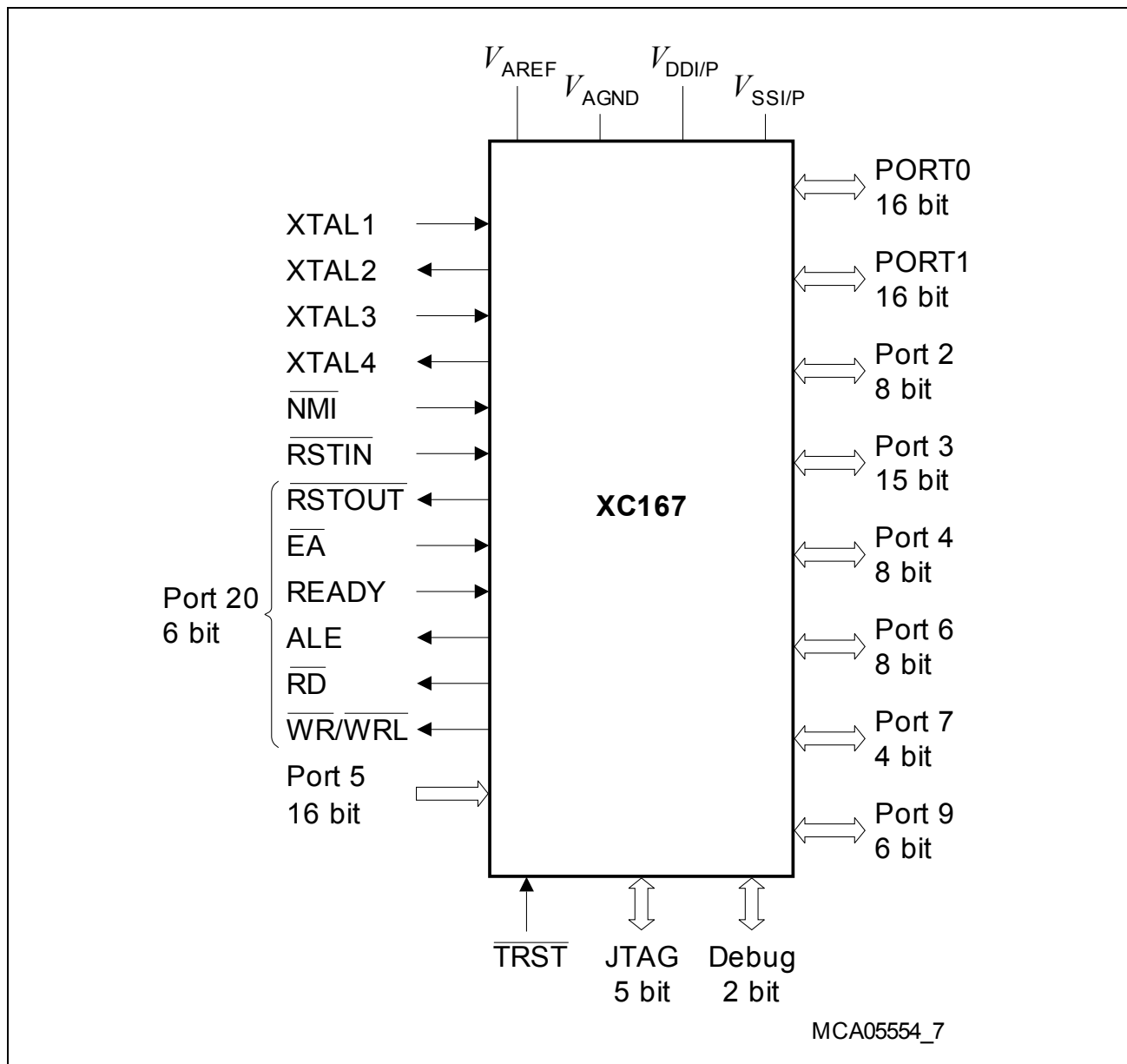
Figure 1 Logic Symbol
