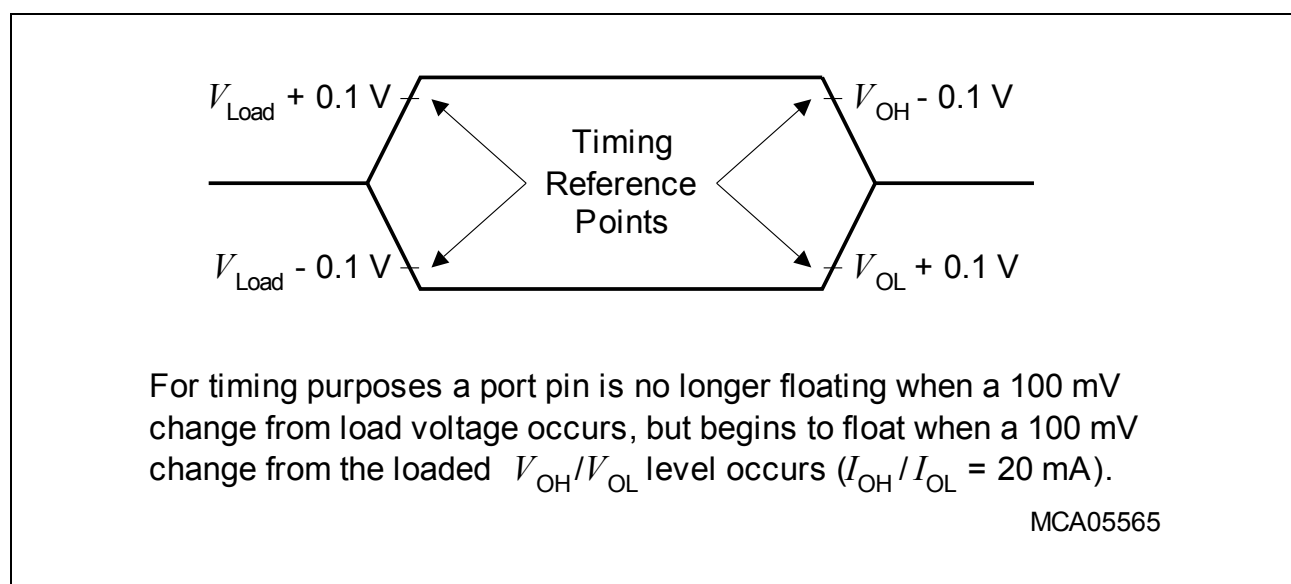
Figure 19 Float Waveforms
