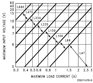
FIGURE 3. LM2576(HV)-3.3
