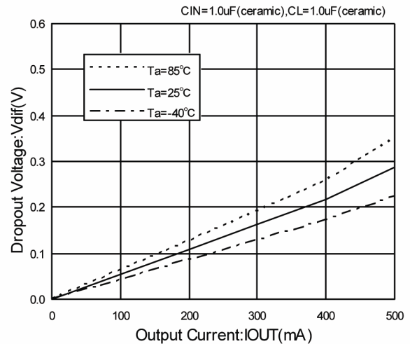
XC6210 (VOUT:2.5V)
