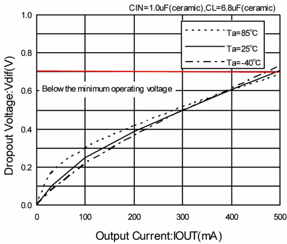
XC6210 (VOUT:0.8V)
