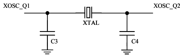
Figure 16. Crystal oscillator circuit
