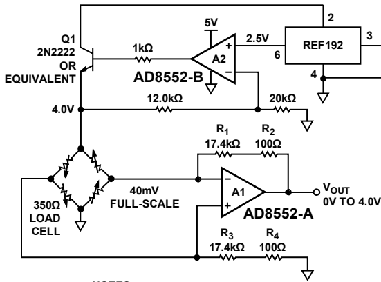
Figure 65. A 5 V Precision Strain Gage Amplifier
