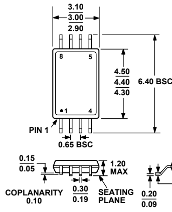
Figure 72. 8-Lead Thin Shrink Small Outline Package [TSSOP] (RU-8)
