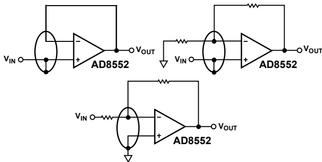
Figure 52. Guard Ring Layout and Connections to Reduce PCB Board Leakage Currents
