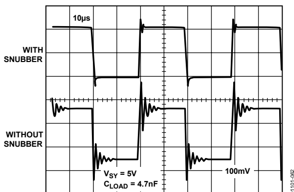
Figure 62. Overshoot and Ringing are Substantially Reduced Snubber Network
