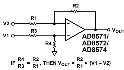
Figure 64. Using the AD857x as a Difference Amplifier
