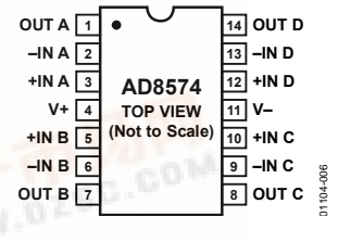
Figure 6. 14-Lead SOIC (R Suffix)
