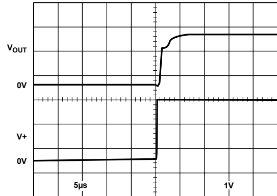
BOTTOM TRACE = 2V/DIV TOP TRACE = 1V/DIV
