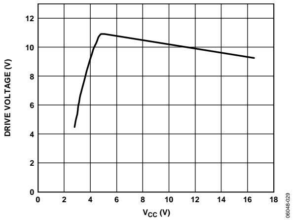
Figure 5. Drive Voltage (V GATE - V CC ) vs. Supply Voltage
