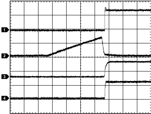
Figure 44. Inrush Current Control into 220 \mu F Load (CH1 = I_{LOAD} , CH2 = V_{TIMER} , CH3 = V_{GATE} , CH4 = V_{OUT} )
