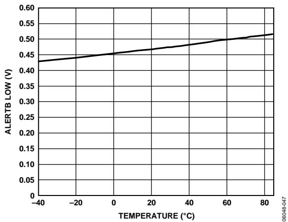
Figure 30. Output Low Voltage vs. Temperature @ 1 mA
