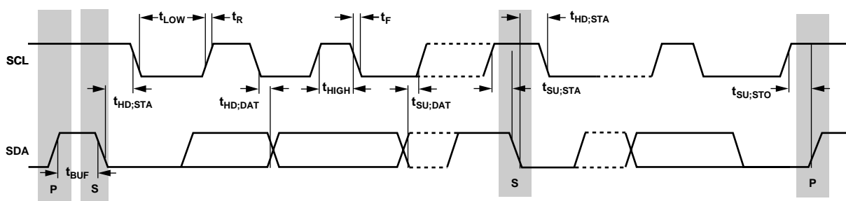
Figure 37. Serial Bus Timing Diagram
