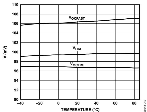
Figure 23. V OCTIM , V LIM , V OFAST vs. Temperature
