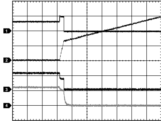
Figure 47. Overcurrent Condition During Operation (ADM1178-1 Model) (CH1 = I_{LOAD} , CH2 = V_{TIMER} , CH3 = V_{GATE} , CH4 = V_{OUT} )
