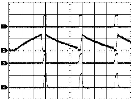
Figure 46. Overcurrent Condition at Startup (ADM1178-2 Model) (CH1 = I_{LOAD} , CH2 = V_{TIMER} , CH3 = V_{GATE} , CH4 = V_{OUT} )
