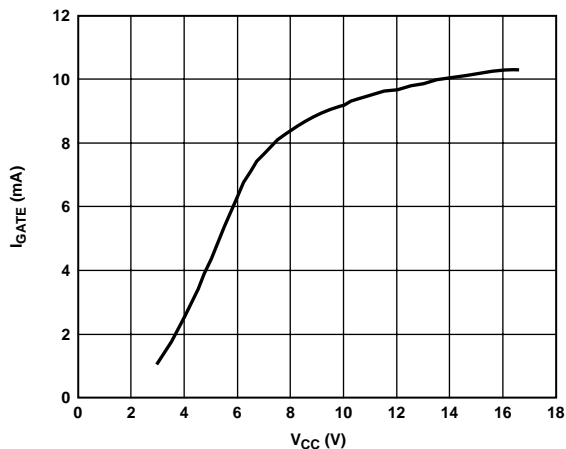
Figure 10. Gate Pull-Down Current vs. V CC at V GATE = 5 V
