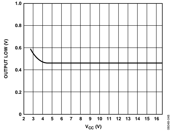
Figure 31. Output Low Voltage vs. Supply @ 1 mA
