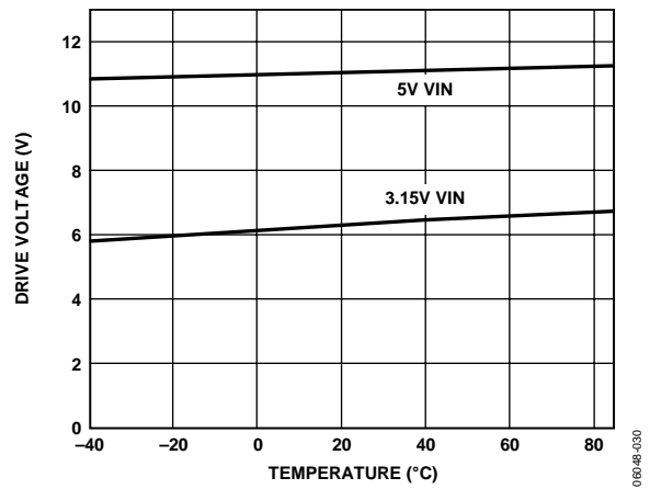
Figure 8. Drive Voltage (V GATE - V CC ) vs. Temperature
