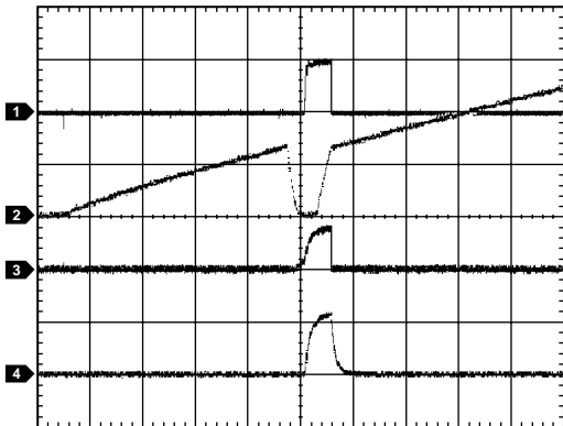
Figure 45. Overcurrent Condition at Startup (ADM1178-1 Model) (CH1 = I_{LOAD} , CH2 = V_{TIMER} , CH3 = V_{GATE} , CH4 = V_{OUT} )
