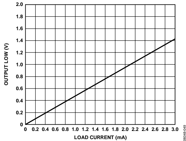
Figure 32. Output Low Voltage vs. Load Current
