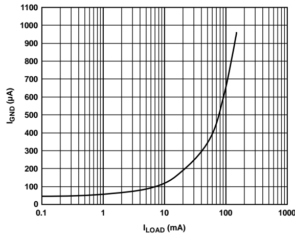
Figure 11. Ground Current vs. Load Current
