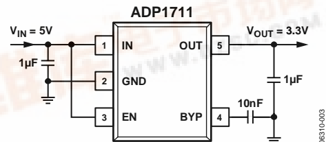
Figure 3. ADP1711 with Fixed Output Voltage and Bypass Capacitor, 3.3 V
