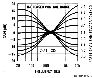
FIGURE 2. Tone Characteristic (Gain vs Frequency)
