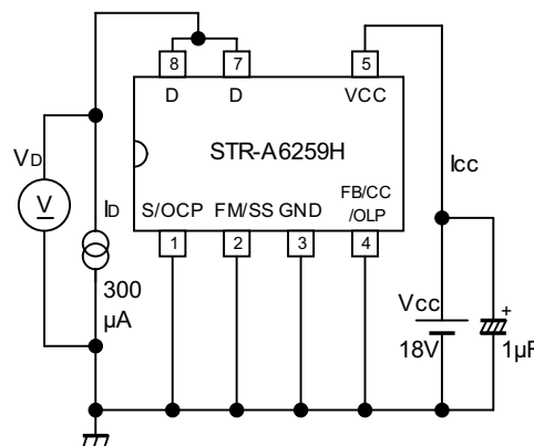
Measurement Circuit 7
