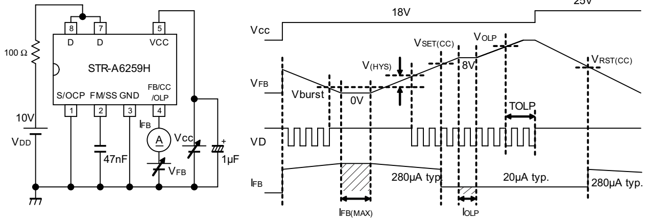
Measurement Circuit 5
