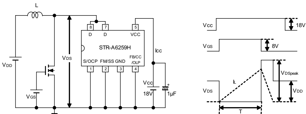
Measurement Circuit 7
