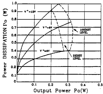
Power Dissipation vs. Output Power (RL=4Ω)
