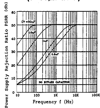
Power Supply Rejection Ratio vs. Frequency (V + =6V, A v =26dB)
