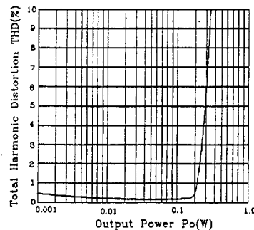
Total Harmonic Distortion vs. Output Power (V + =6V, R L =8Ω, f=1KHz)
