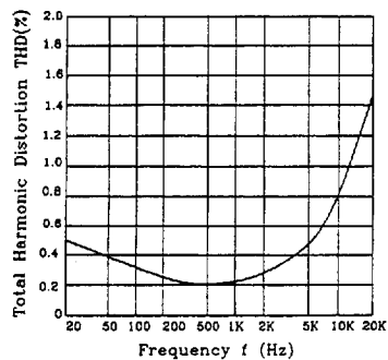
Total Harmonic Distortion vs. Frequency (V + =6V, R L =8Ω, P o =125mW, A v =26dB)
