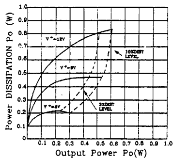
Power Dissipation vs. Output Power (RL=8Ω)
