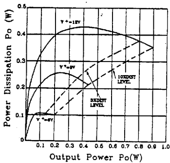
Power Dissipation vs. Output Power (RL=16Ω)
