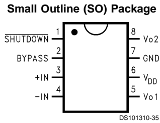
Top View Order Number LM4890M See NS Package Number M08A
