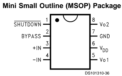
Top View Order Number LM4890MM See NS Package Number MUA08A
