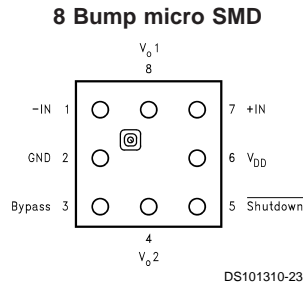
Top View Order Number LM4890IBP, LM4890IBPX See NS Package Number BPA08FFB
