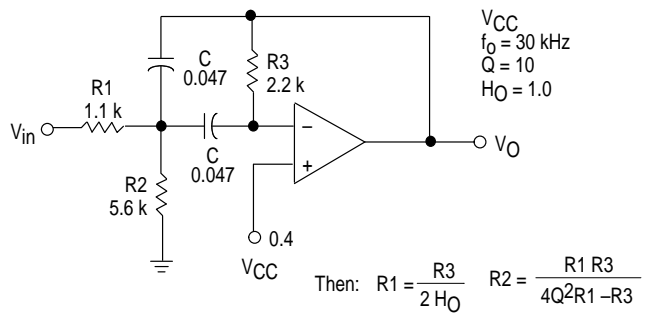
Figure 14. Active Bandpass Filter
