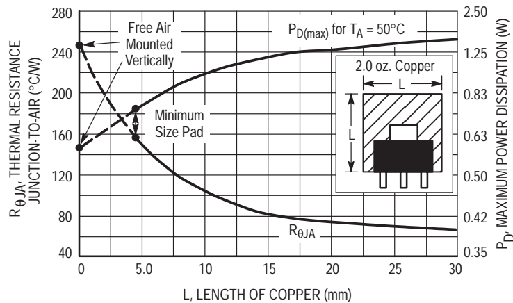
Figure 24. SOT-223 Thermal Resistance and Maximum Power Dissipation versus P.C.B. Copper Length
