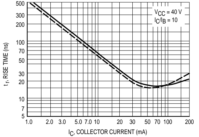
Figure 6. Rise Time
