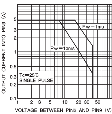
Fig.19 Safe operation range (ASO)
