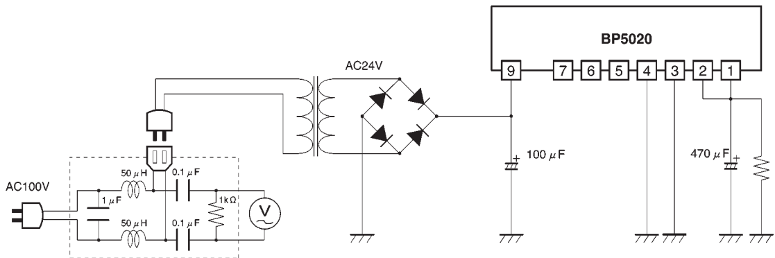
Fig.10 Measurement circuit
