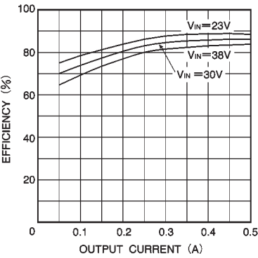
Fig.18 Efficiency
