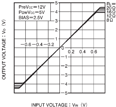
Fig. 14 Driver I/O characteristics (loading)
