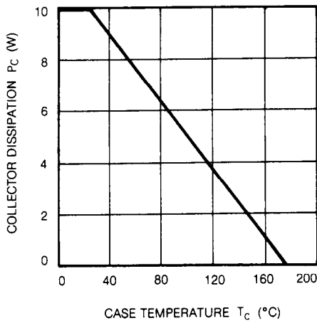
COLLECTOR DISSIPATION VS. CASE TEMPERATURE
