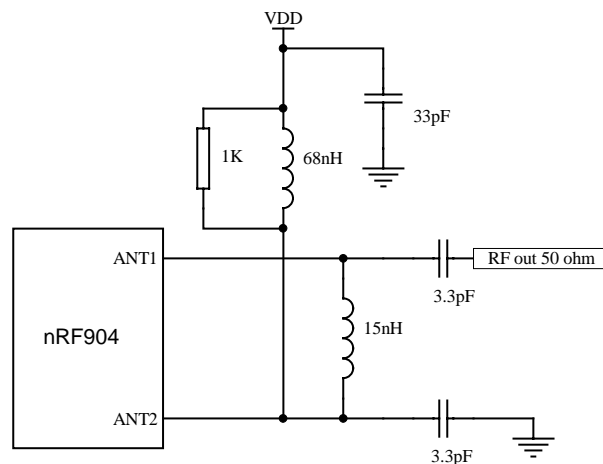
Figure 8. Connection of nRF904 to single ended antenna (50 Ω) by using a differential to single ended matching network.
