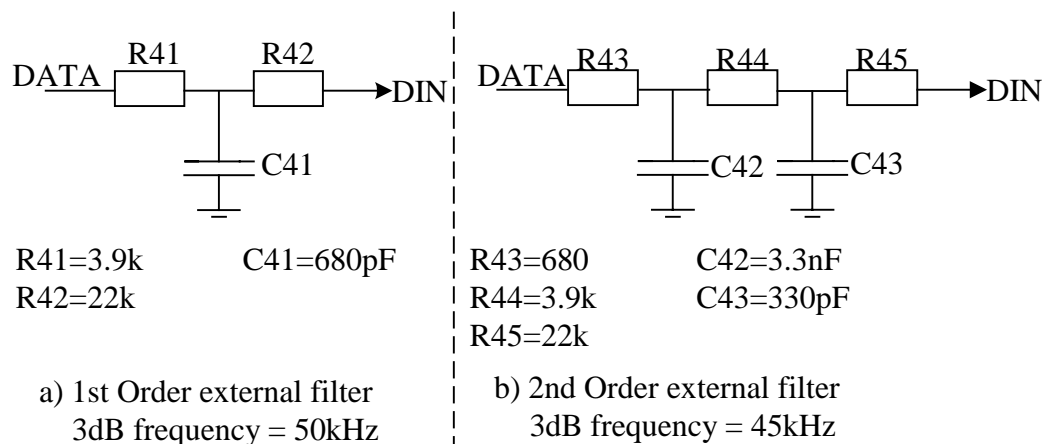
Figure 5. Alternative external DIN components for setting the spectral bandwidth.
