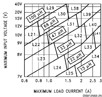
FIGURE 5. LM2596-5.0
