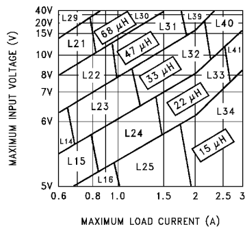
FIGURE 4. LM2596-3.3
