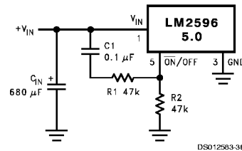
FIGURE 21. Delayed Startup
