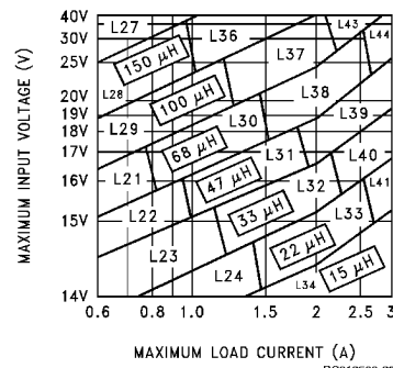
FIGURE 6. LM2596-12
