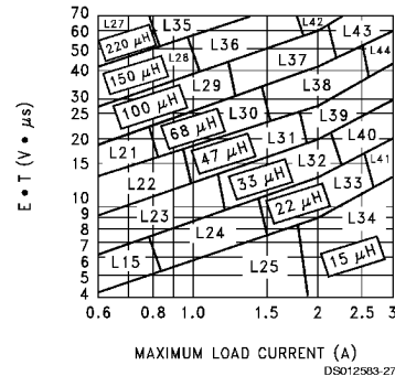
FIGURE 7. LM2596-ADJ
