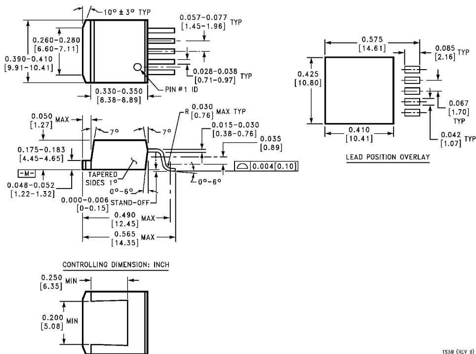
5-Lead TO-263 Surface Mount Package (S) Order Number LM2596S-3.3, LM2596S-5.0, LM2596S-12 or LM2596S-ADJ NS Package Number TS5B
