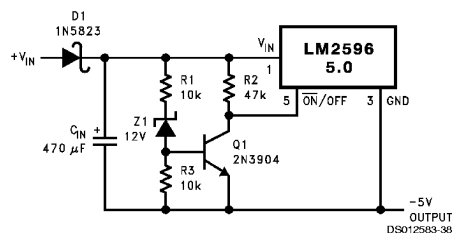
FIGURE 23. Undervoltage Lockout for Inverting Regulator
