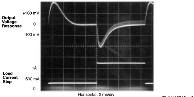
TL/H/12316-12 FIGURE 6. V OUT Load Current Step Response
