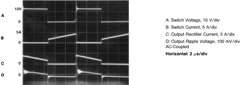
TL/H/12316-11 FIGURE 5. Switching Waveforms
