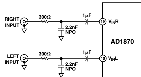
Figure 2. Recommended Input Structure for Externally DC-Coupled Inputs
