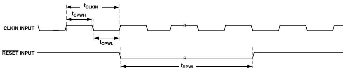
Figure 19. CLKIN and RESET Timing
