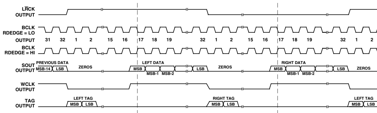
Figure 11. Serial Data Output Timing: Master Mode, Right-Justified with No MSB Delay, S^M = LO , R^LJUST = HI , \overline{MSBDLY} = HI
