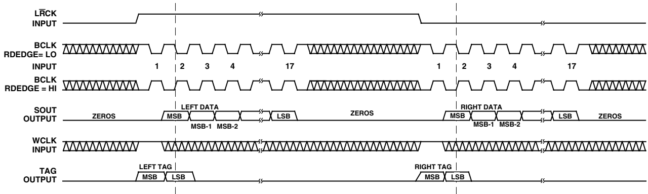
Figure 8. Serial Data Output Timing: Slave Mode, Data Position Controlled by WCLK Input, S\overline{M} = HI , R\overline{L}JUST = HI , \overline{MSBDLY} = LO
