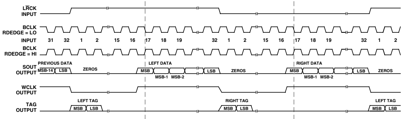
Figure 7. Serial Data Output Timing: Slave Mode, Right-Justified with No MSB Delay, S\overline{M} = HI , R\overline{L}JUST = HI , \overline{MSBDLY} = HI
