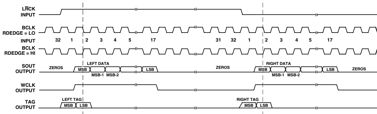
Figure 10. Serial Data Output Timing: Slave Mode, P 2 S-Justified, S^M = HI , R^LJUST = LO , \overline{MSBDLY} = LO
