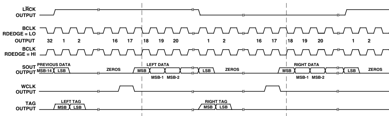
Figure 12. Serial Data Output Timing. Master Mode, Right-Justified with MSB Delay, WCLK Pulsed in 17th BCLK Cycle, S^M = LO , R^LJUST = HI , \overline{MSBDLY} = LO
