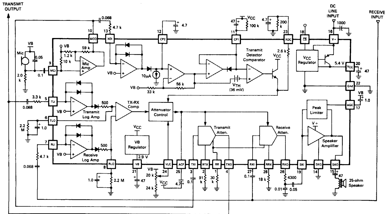
FIGURE 1 — TEST CIRCUIT
