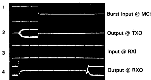
FIGURE 16 — TRANSMIT-RECEIVE SWITCHING
